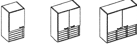
form cabinet - CWFDF W - 12,16,18,20,24,28,30,32,36 H - 18,24,30,36,40 D - 14
