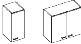
wall cabinet w/doors - CW W - 12,16,18,20,24, 28,30,32,36 H - 18,24,30,36,40 D - 14
