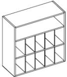
lateral storage - CWLSF323614 W - 32 H - 36 D - 14 (actual 13.125) includes 10 slots
