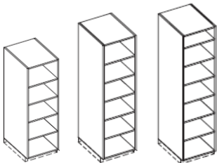
open cabinet - CCAB W - 12,16,18,20,24,28,30,32,36 H - 61,71,80 D - 14,20,24 (actual 13.125, 19.125, 23.125)
