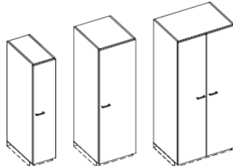
storage cabinet w/doors - CSC W - 12,16,18,20,24,28,30,32,36 H - 61,71,80 D - 14,20,24
