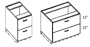
file base - CFB
