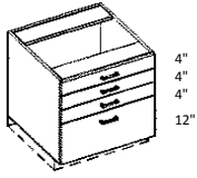
utility base - CUDB
